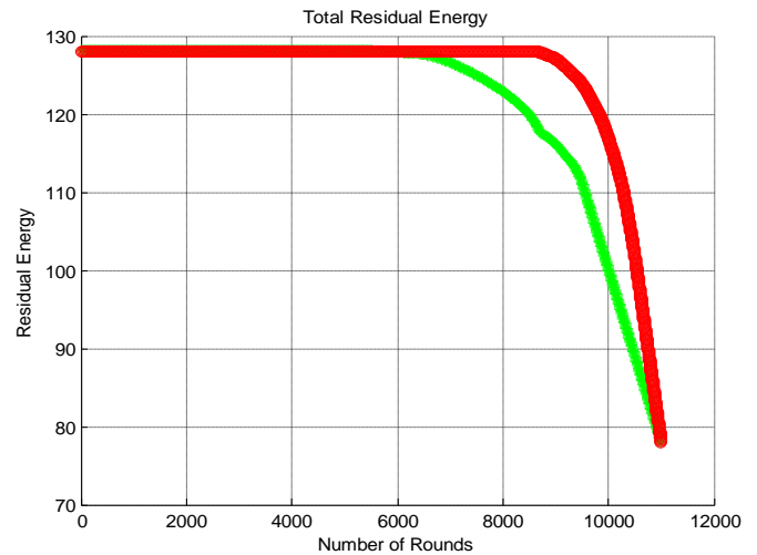
Figure 3: Output of the FAF routing and proposed system using residual energy monitoring
