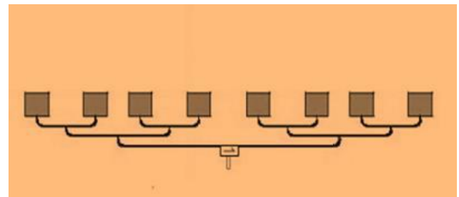
Figure 4: Design of RO3006 for Microstrip feed Array.
