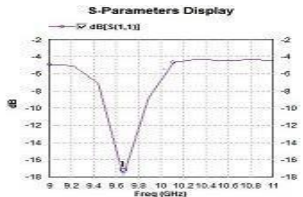
Figure 5: s-parameter plot of array.
