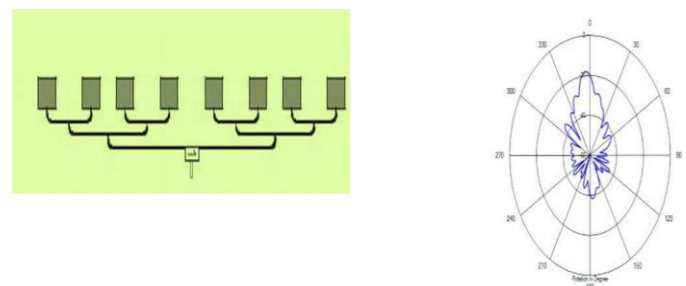
Figure 1: Design of FR4 for Microstrip feed Array.
