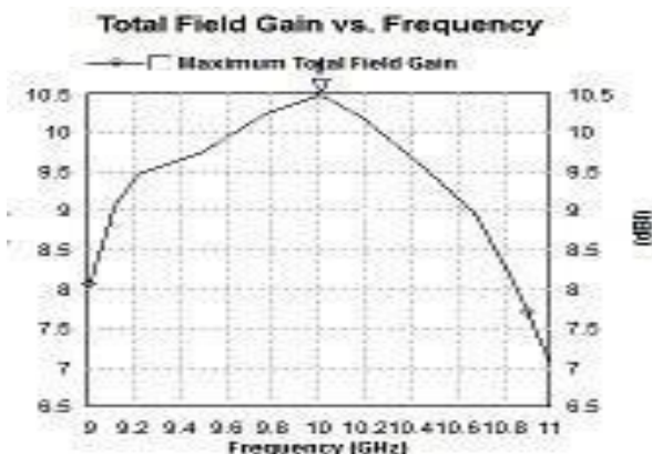
Figure 3: Gain vs frequency plot.
