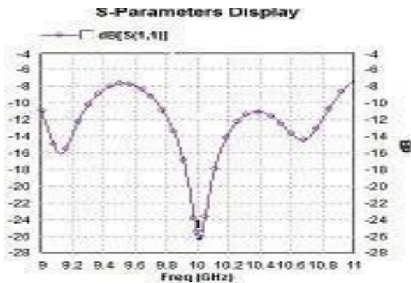
Figure 2: s-parameter plot of array.
