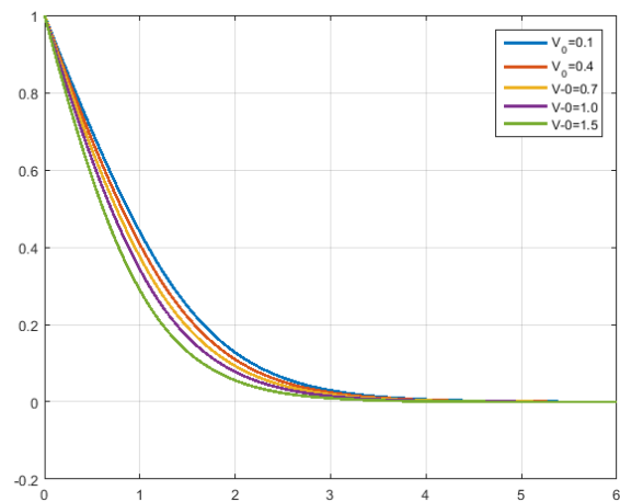
Figure 5: Effect of V_0 on concentration profile by the proposed method.
