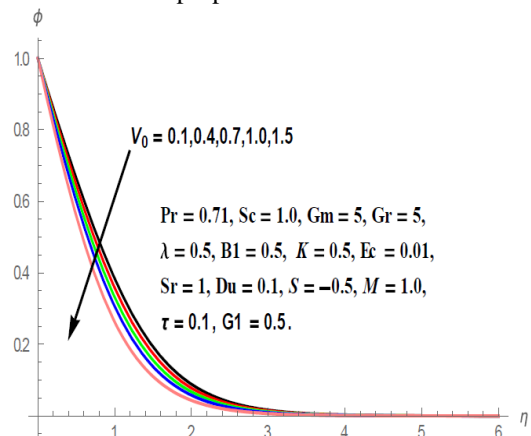
Figure 6: Effect of V_0 on concentration profile in the paper Sudarsana Reddy et.al.(2016).
