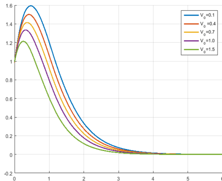
Figure 1: Effect of V_0 on velocity profile by proposed method
