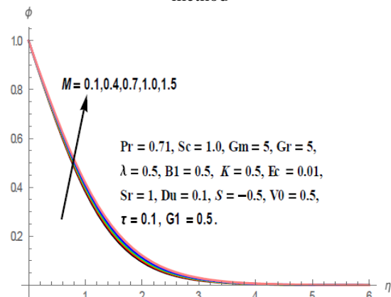
Figure 12: Effect of M on concentration profile in the paper Sudarsana Reddy et.al.(2016).
