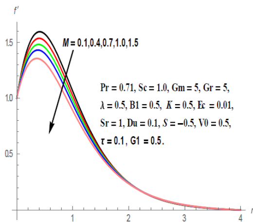
Figure 7: Effect of M on velocity profile by proposed method
