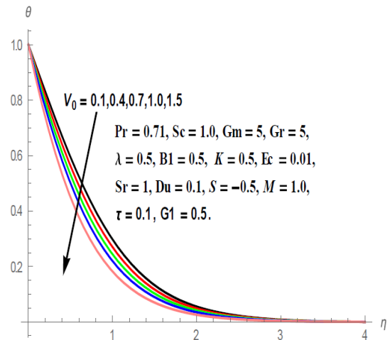
Figure 4: Effect of V_0 on temperature profile in the paper Sudarsana Reddy et.al.(2016)
