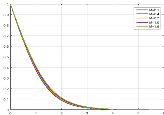
Figure 11: Effect of M on concentration profile by proposed method
